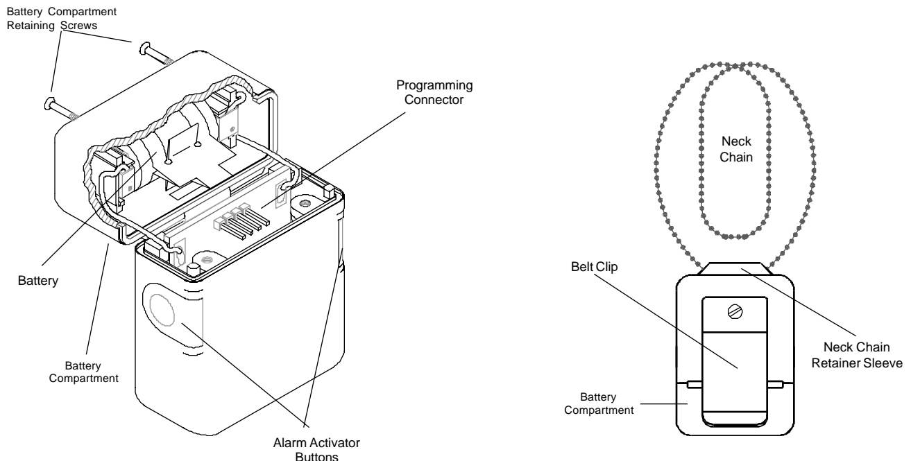
Figure 1 - Transmitter Housing
